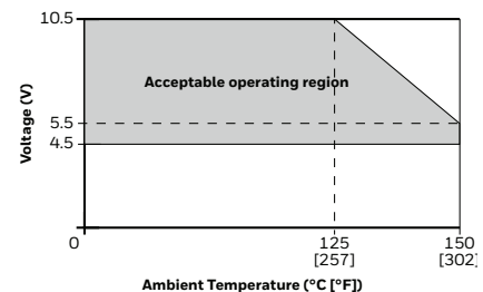
FIGURE 2. MAXIMUM SUPPLY VOLTAGE VS TEMPERATURE
