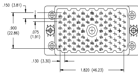
90 PIN PLUG
