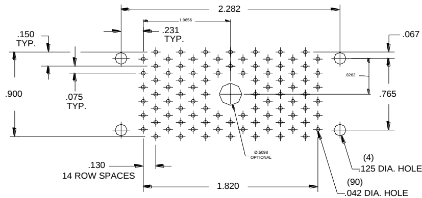
90 PINS
