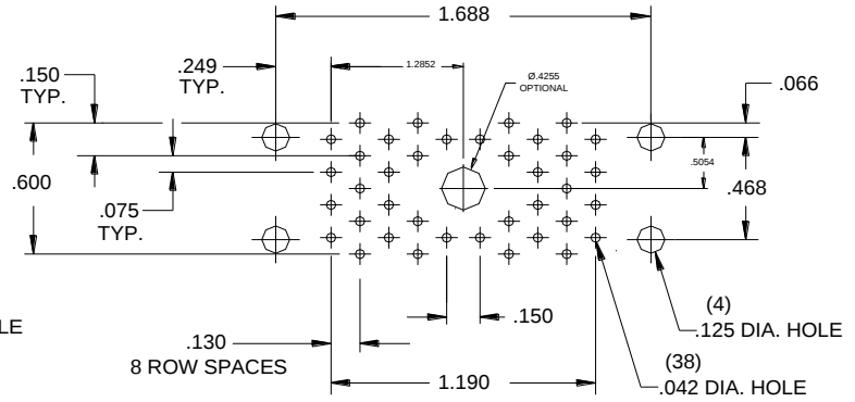
38 PINS
