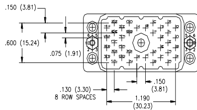
38 PIN PLUG
