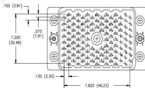
120 PIN PLUG
