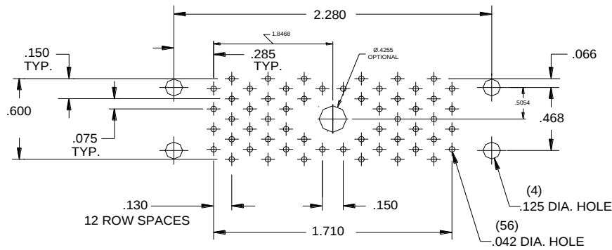
56 PINS
