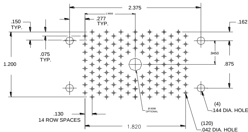
120 PINS
