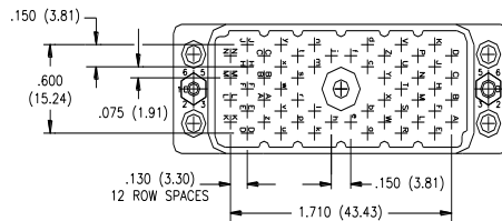
56 PIN PLUG
