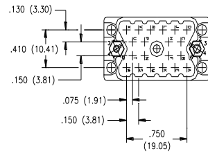
20 PIN PLUG
