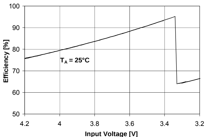
Efficiency for 6 LEDs at 10mA and 3.31V
