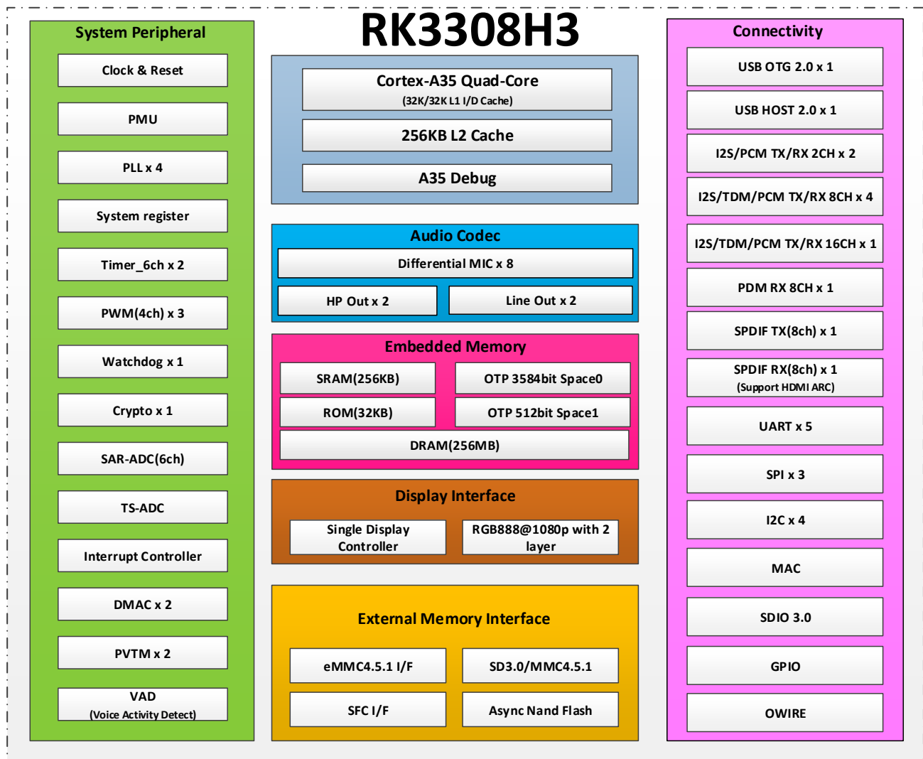
Fig.1-1 RK3308H3 Block Diagram
