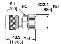
N Series Plug to 7 mm Best VSWR Jack
