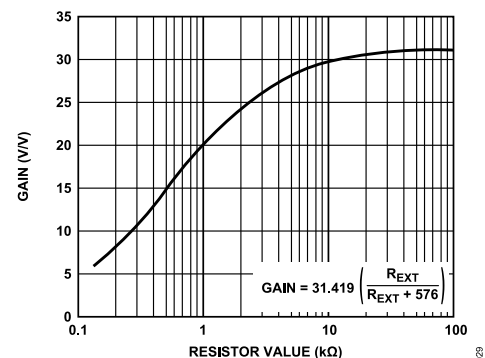
Figure 20. Gain vs. External Resistor Value
