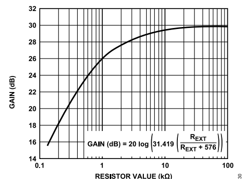
Figure 21. Gain (dB) vs. External Resistor Value
