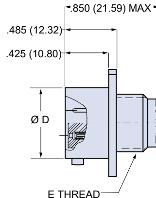
Accessory Thread 803-004-02
