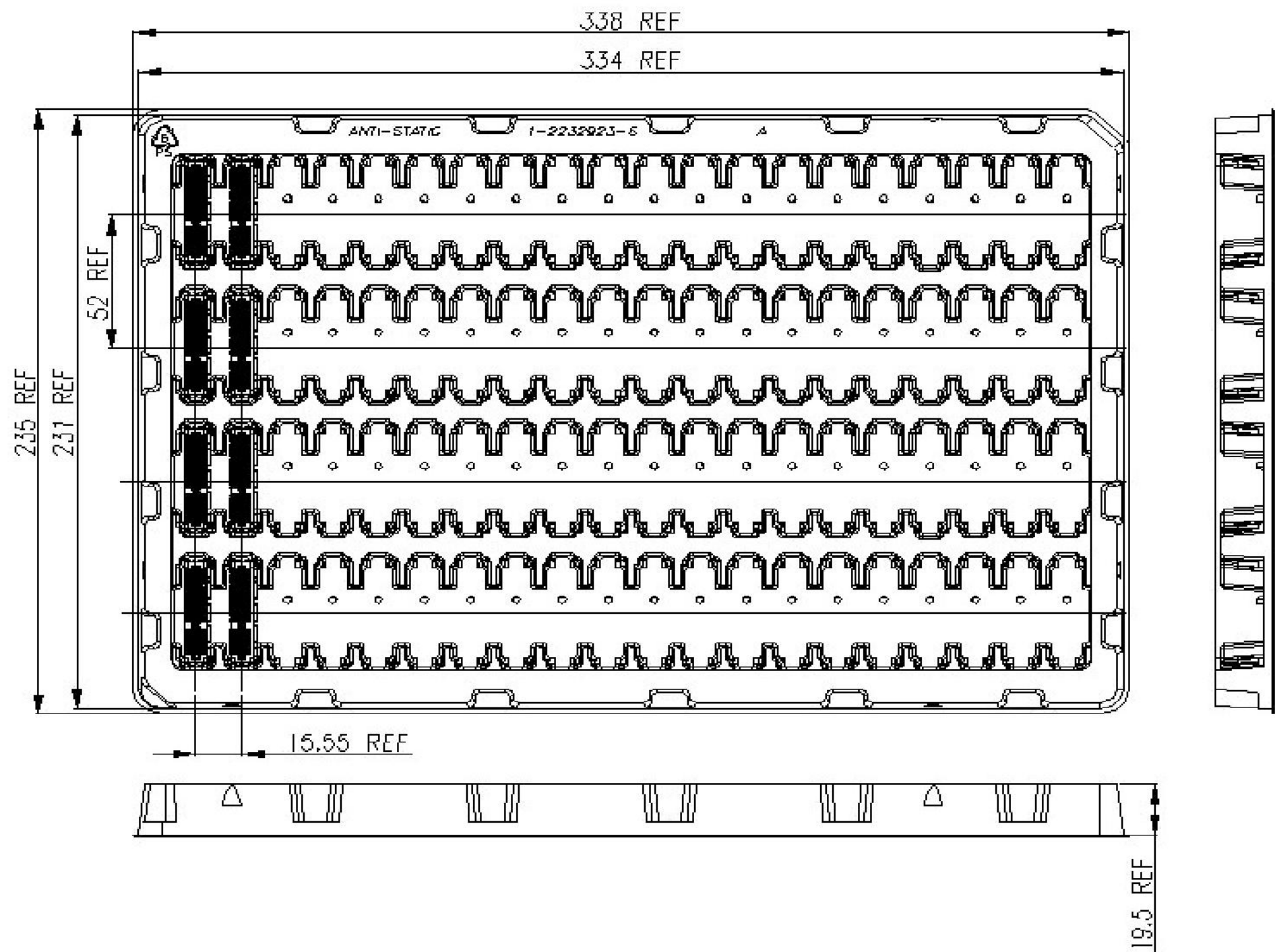
SOFT TRAY: FOR 64POS SCALE 1:2
