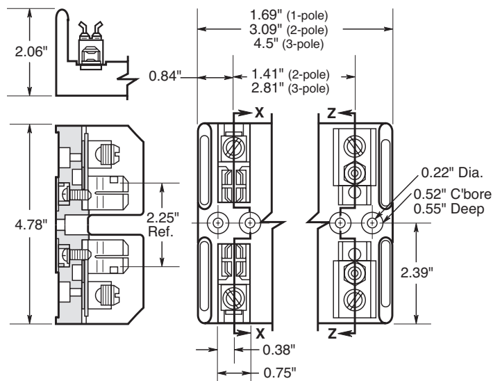
Figure 2. 61 to 100A
