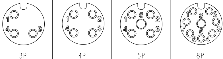
Pin Assignments Front View
