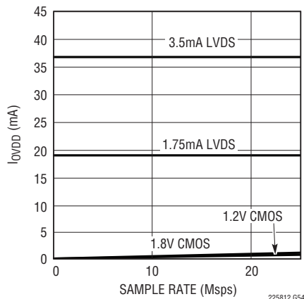
LTC2256-12: I_{OVPD} vs Sample Rate, 5MHz Sine Wave Input, -1dB, 5pF on Each Data Output
