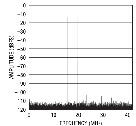
LTC2206-14: 32K Point 2-Tone FFT, f_{IN} = 14.87MHz and 18.56MHz, -15dBFS, PGA = 0, RAND = "On", Dither "Off"
