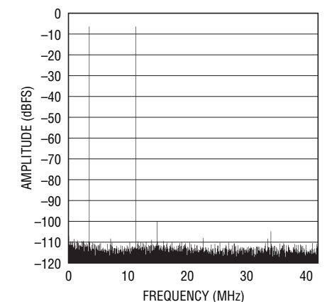
LTC2206-14: 32K Point 2-Tone FFT, f_{IN} = 69.2MHz and 76.5MHz, -7dBFS, PGA = 0, RAND = "On", Dither "Off"
