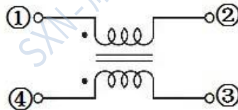
Schematic Diagram
