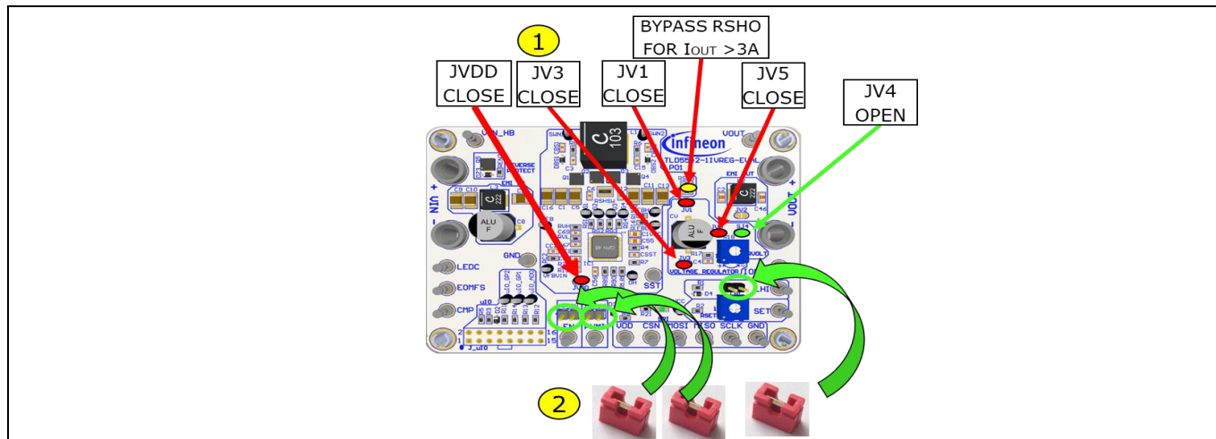
Figure 6 Voltage regulator , set LHI and EN jumpers, populate solder jumps
