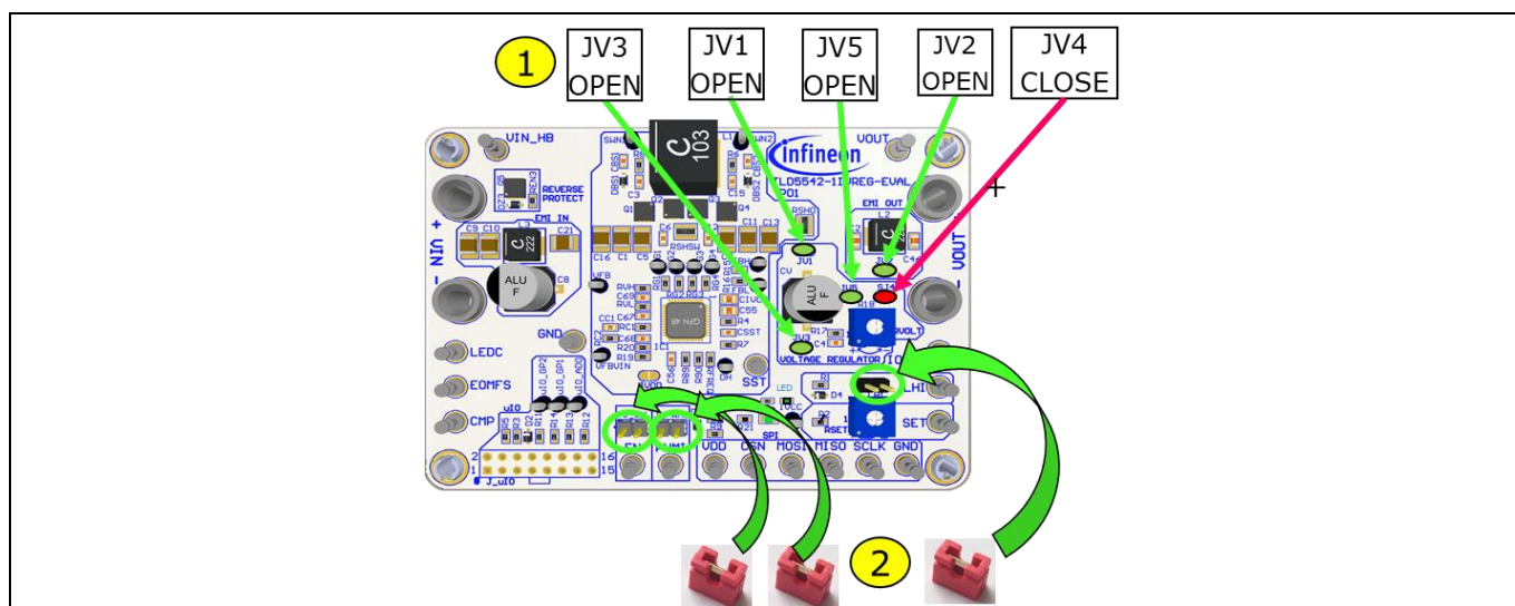
Figure 4 Connect loads and set jumpers for limp home
