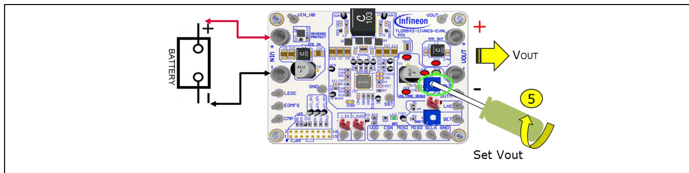
Figure 8 Adjust V_{OUT} using RVOLT
