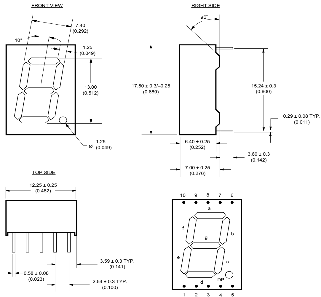
Figure 2: HDSP-561x/563x Series
