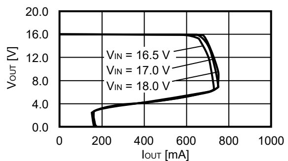
1.4 V_{\text{OUT}} = 16.0 \text{ V}
