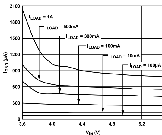
Figure 15. Ground Current ( I_{GND} ) vs. Input Voltage ( V_{IN} )
