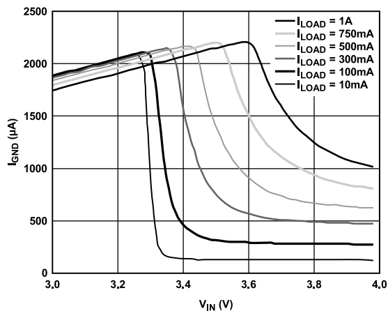
Figure 18. Ground Current ( I_{\text{GND}} ) vs. Input Voltage ( V_{\text{IN}} ) (in Dropout)
