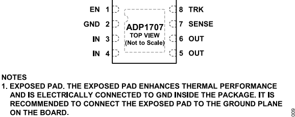
Figure 7. 8-Lead LFCSP, ADP1707
