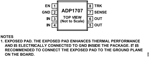
Figure 6. 8-Lead SOIC, ADP1707
