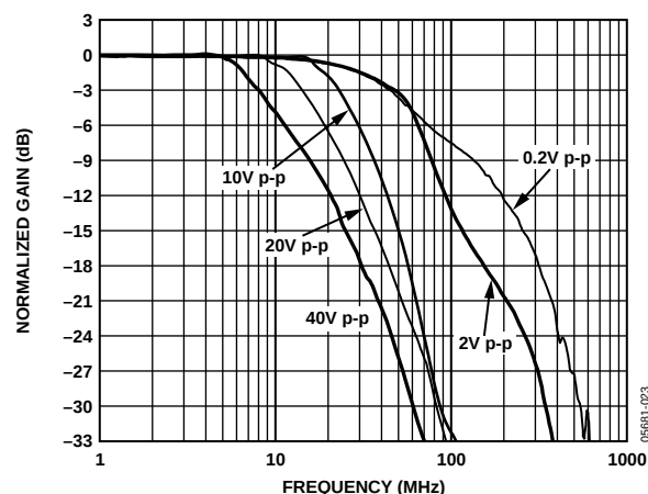
Figure 15. Frequency Response for Various Output Amplitudes, V_S = \pm 12 V
