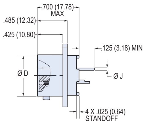
Flange Mount Receptacle 803-005-02
