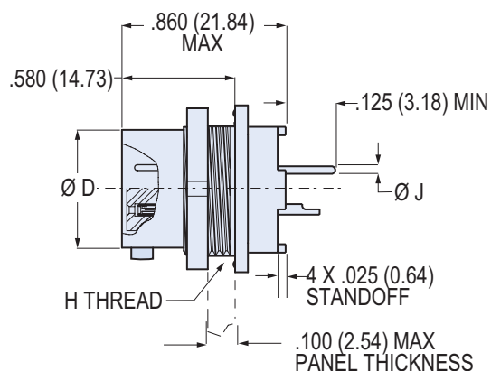
Jam Nut Receptacle 803-005-07
