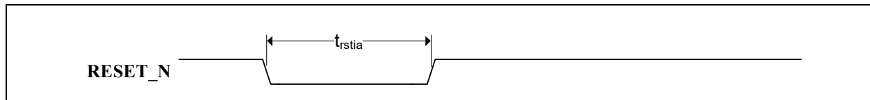
FIGURE 5-2: RESET_N TIMING
