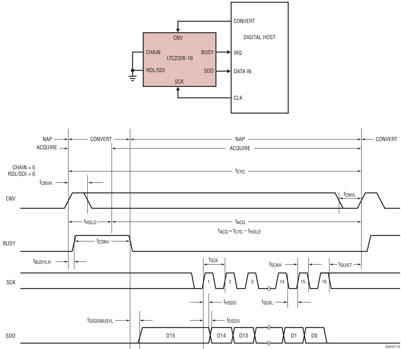
Figure 10. Using a Single LTC2326-16 in Normal Mode
