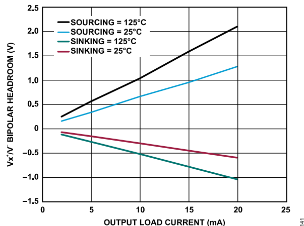
Figure 45. V x + /V - Bipolar Headroom vs. Output Load Current
