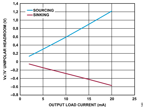
Figure 44. V x + /V - Unipolar Headroom vs. Output Load Current
