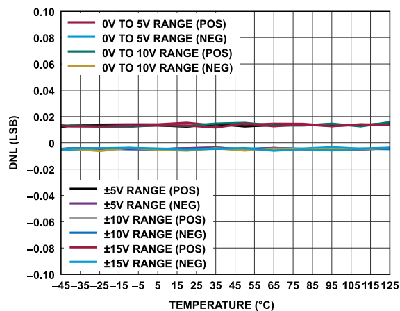
Figure 33. LTC2688-12 DNL vs. Temperature
