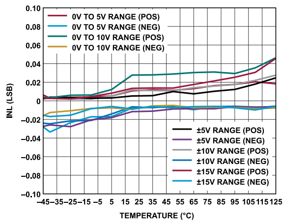
Figure 32. LTC2688-12 INL vs. Temperature
