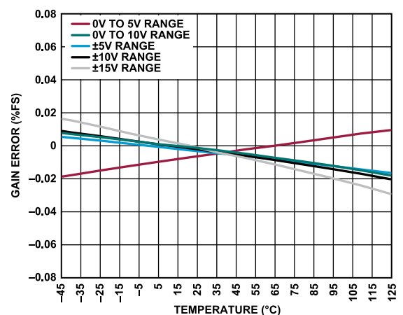
Figure 34. Gain Error vs. Temperature
