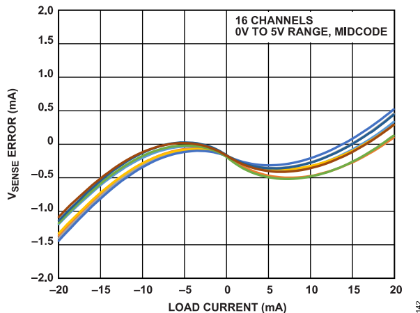
Figure 46. V SENSE Error vs. Load Current from Equation 5
