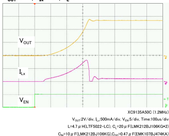
V_{OUT}=5.0\text{V} , V_{IN}=5.5\text{V} , R_L=50\Omega
