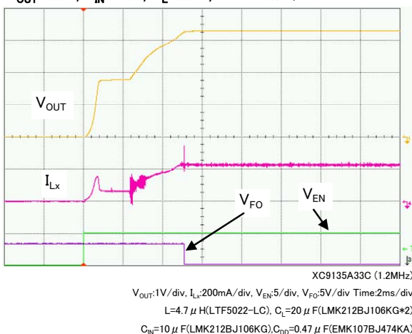
V_{OUT}=3.3\text{V} , V_{IN}=1.8\text{V} , R_L=33\Omega , MODE:PWM/PFM
