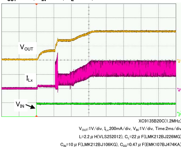
V_{OUT}=2.0\text{V} , V_{IN}=0.9\text{V} , R_L=20\Omega , MODE:PWM/PFM
