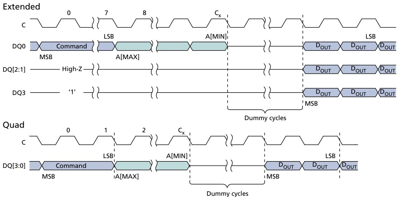
Figure 15: QUAD OUTPUT FAST READ – 6Bh/6Ch 3
