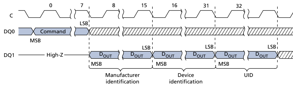
Figure 10: READ ID and MULTIPLE I/O READ ID Commands
