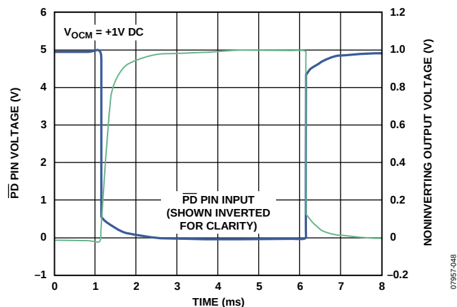
Figure 48. \overline{PD} Response Time
