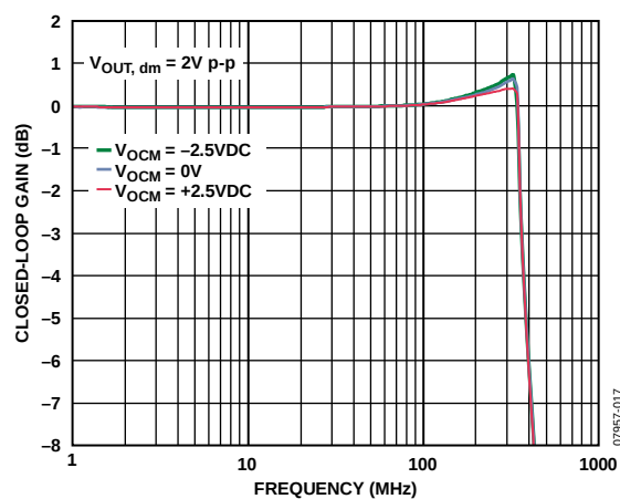
Figure 17. Large-Signal Frequency Response for Various V_{OCM} Levels
