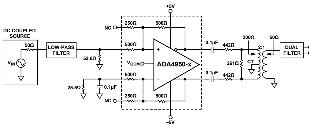
Figure 51. Test Circuit for Distortion Measurements
