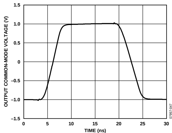
Figure 47. V_{OCM} Large-Signal Pulse Response
