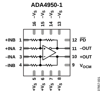
Figure 1. ADA4950-1
