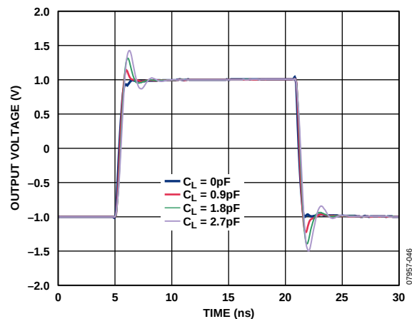
Figure 46. Large-Signal Pulse Response for Various Capacitive Loads
