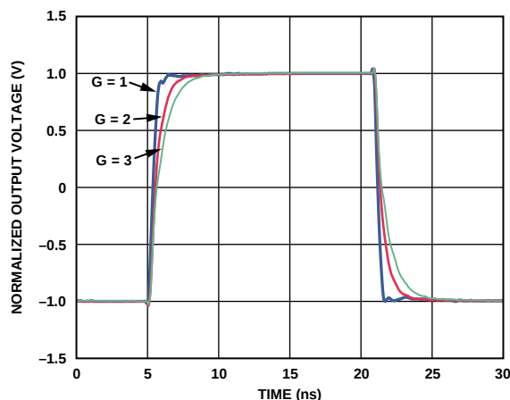
Figure 42. Large-Signal Pulse Response for Various Gains
