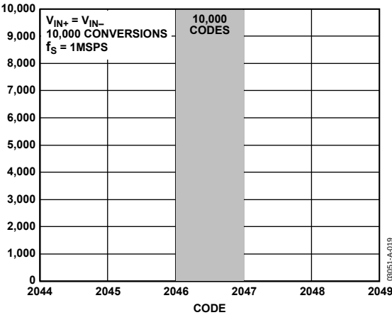
Figure 19. Histogram of 10,000 Conversions of a DC Input for the AD7450A with V_{DD} = 5\text{ V}
