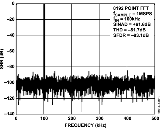
Figure 20. AD7440 Dynamic Performance with V_{DD} = 5\text{ V}
