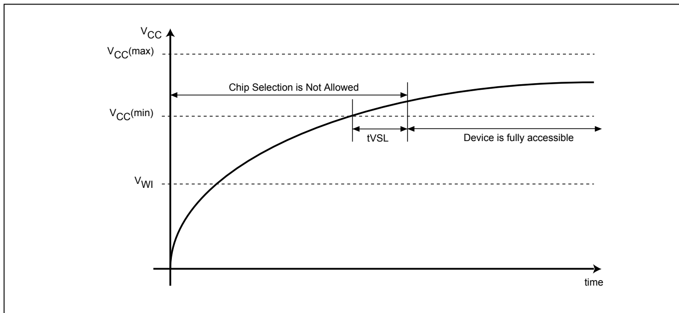
Figure 83. Power-up Timing
