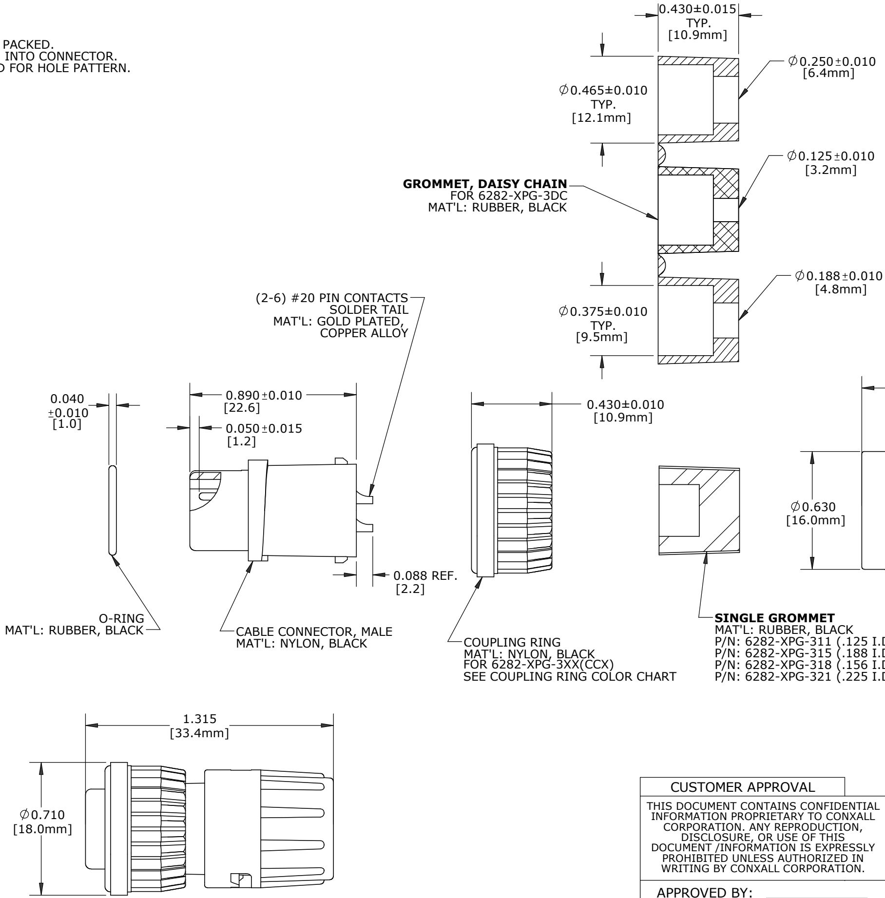
FACE VIEW 6282-2PG-3DC 6282-2PG-3XX
