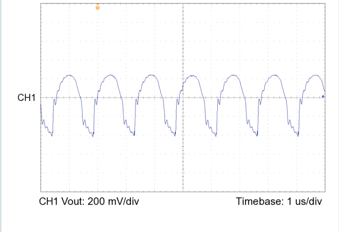
Figure 16 — Output voltage ripple, V_{IN} = 300\text{ V} , V_{OUT} = 12.0\text{ V} , C_{OUT\_EXT} = 1000\text{ }\mu\text{F} , R_{LOAD} = 0.359\text{ }\Omega
