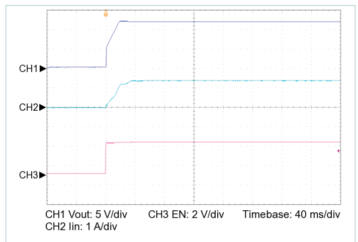
Figure 14 — Startup from EN, V_{IN} = 300\text{ V} , C_{OUT\_EXT} = 10000\text{ }\mu\text{F} , R_{LOAD} = 0.359\text{ }\Omega
