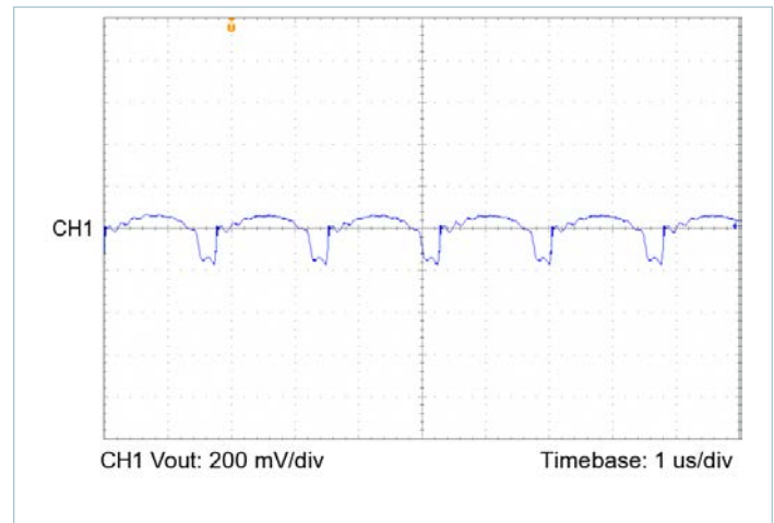
Figure 18 — Output voltage ripple, V_{IN} = 30\text{V} , V_{OUT} = 3.3\text{V} , C_{OUT\_EXT} = 1000\mu\text{F} , R_{LOAD} = 0.136\Omega
