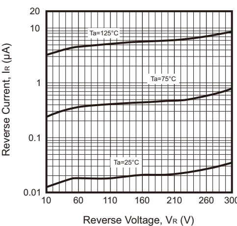
Fig.4 - Reverse Characteristics
