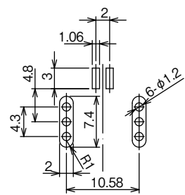
Recommended PCB Dimensions
