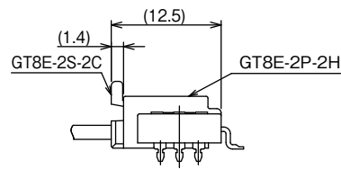
Diagram of Mating Condition During Use
