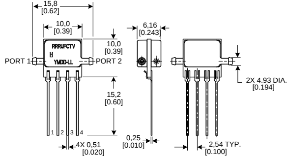
Figure 6. SIP Package Dimensional Drawings (continued)
