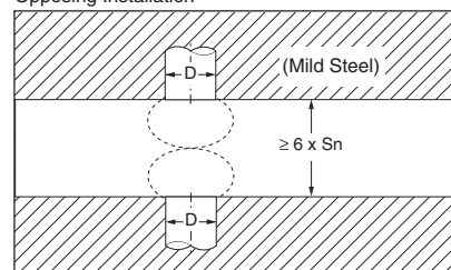
Opposing Installation
