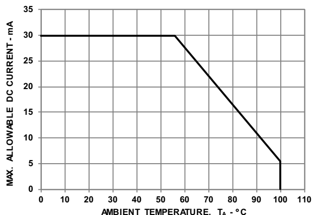
Figure 19: Maximum Forward Current vs. Ambient Temperature for AlInGaP (Derated based on T_{JMAX} = 110 °C, R_{\theta JA} = 750 °C/W)
