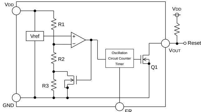
Fig.15 (BD45Exxxx-M Type Internal Block Diagram)
