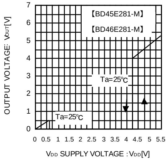
Fig.6 I/O Characteristics
