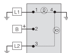
SPDT On-Off-On or On-On dependent (4 terminals)
