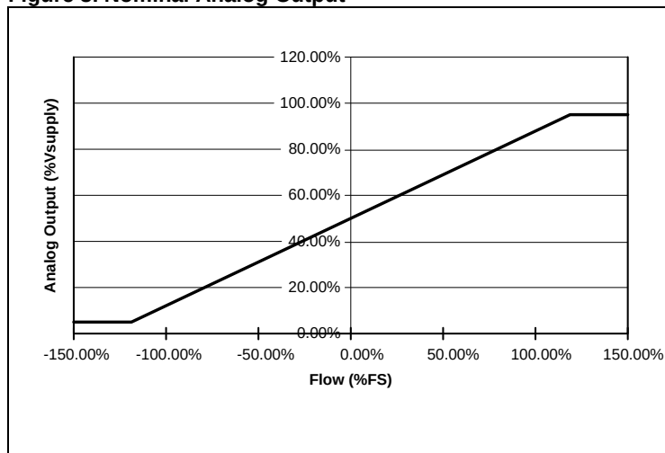
Figure 3. Nominal Analog Output
