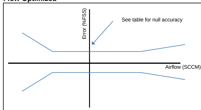
Figure 1. Accuracy Error Band for Bidirectional Forward Flow Optimized
