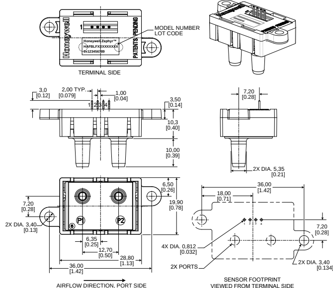
Figure 8. Mounting Dimensions (For reference only: mm [in]). Additional port and housing styles are available.
