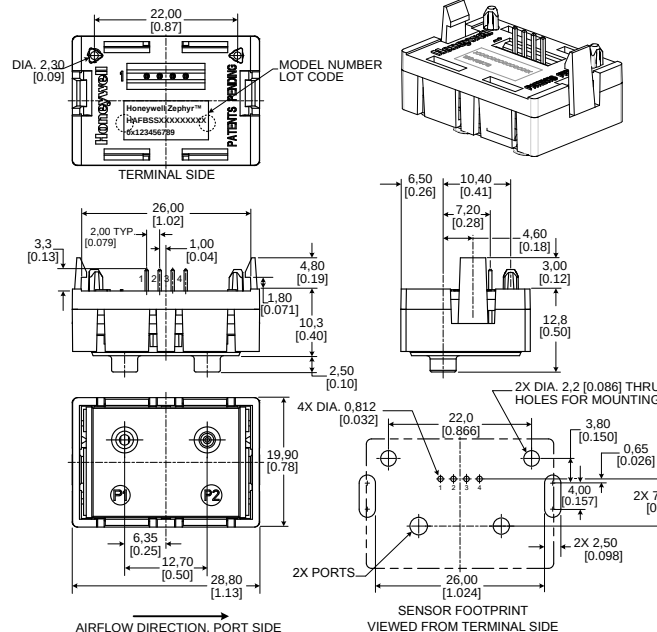
Figure 8. Mounting Dimensions (For reference only: mm [in]). Additional port and housing styles are available.
