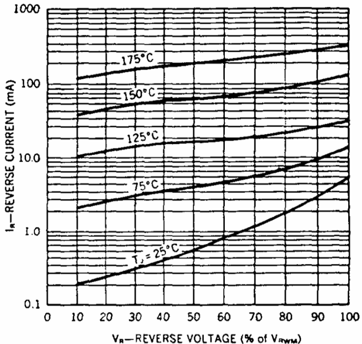
Typical Reverse Current vs Reverse Voltage
