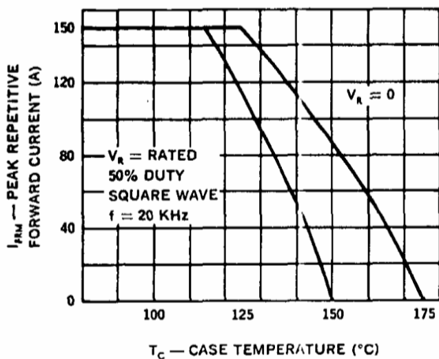
Maximum Current vs Case Temperature
