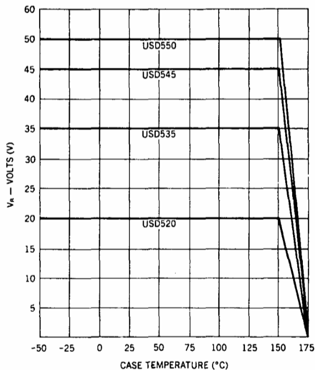
V_{R(MAX)} Rating vs Case Temperature
