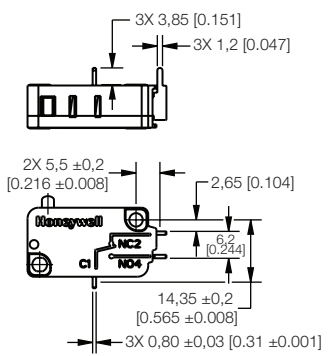
Figure 16. V15 Series R-style Right-Side PCB Terminal
