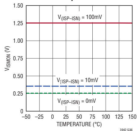
ISMON vs Temperature
