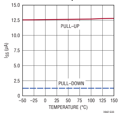
SS Current vs Temperature
