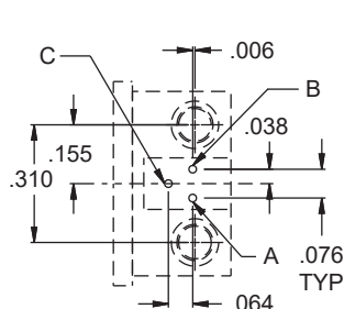
ARRANGEMENT NO. 5-3 (3 #23 CONTACTS)
