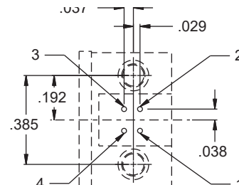
ARRANGEMENT NO. 6-4 (4 #23 CONTACTS)
