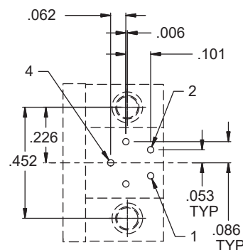
ARRANGEMENT NO. 6-4 (4 #23 CONTACTS)
