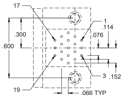
ARRANGEMENT NO. 9-19 (19 #23 CONTACTS)
