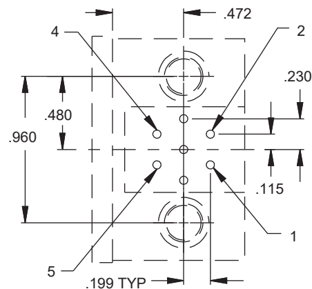
ARRANGEMENT NO. 17-7 (7 #12 CONTACTS)
