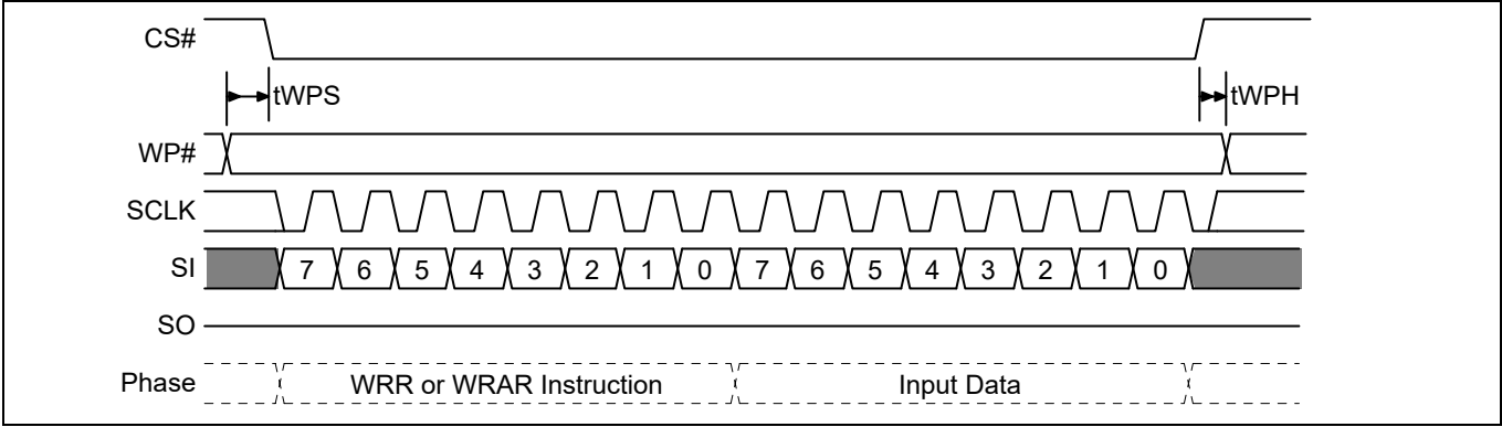
Figure 34 WP# input timing
