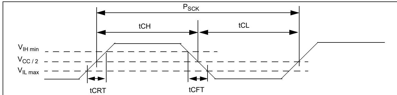
Figure 30 Clock timing
