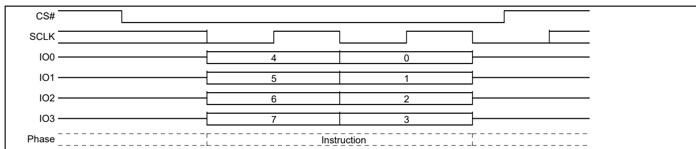
Figure 58 Write Disable (WRDI) command sequence QPI mode
