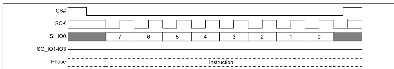
Figure 57 Write Disable (WRDI) command sequence
