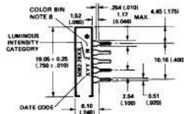
C SIDE
