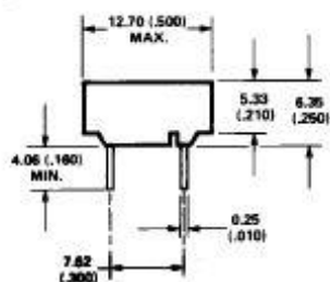
END VIEW
