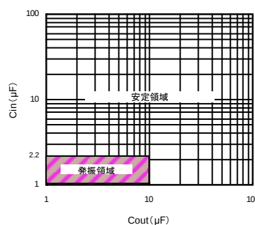
Cin vs Cout 1.0V \leq V_O < 3.0V Cout and Ceramic capacitor 10 \mu F is connected in parallel. (Reference data)
