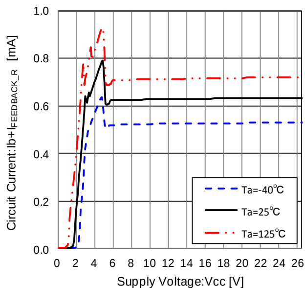
Figure 11. Circuit Current ( I_{FEEDBACK\_R}^{(Note\ 1)} \approx 75\mu A )
