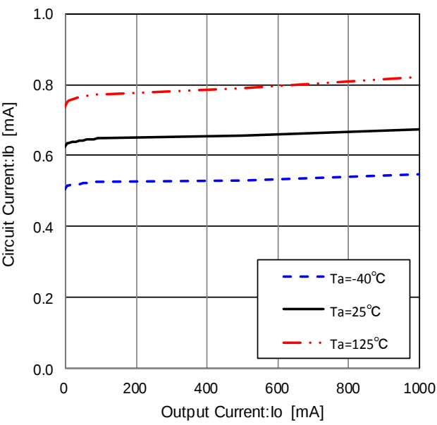
Figure 54. Circuit Current
