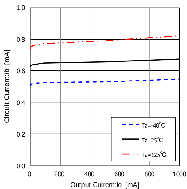
Figure 30. Circuit Current
