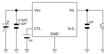
Measurement setup for Figure 25, 36, 48 and 60
