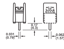
08 Printed Circuit
