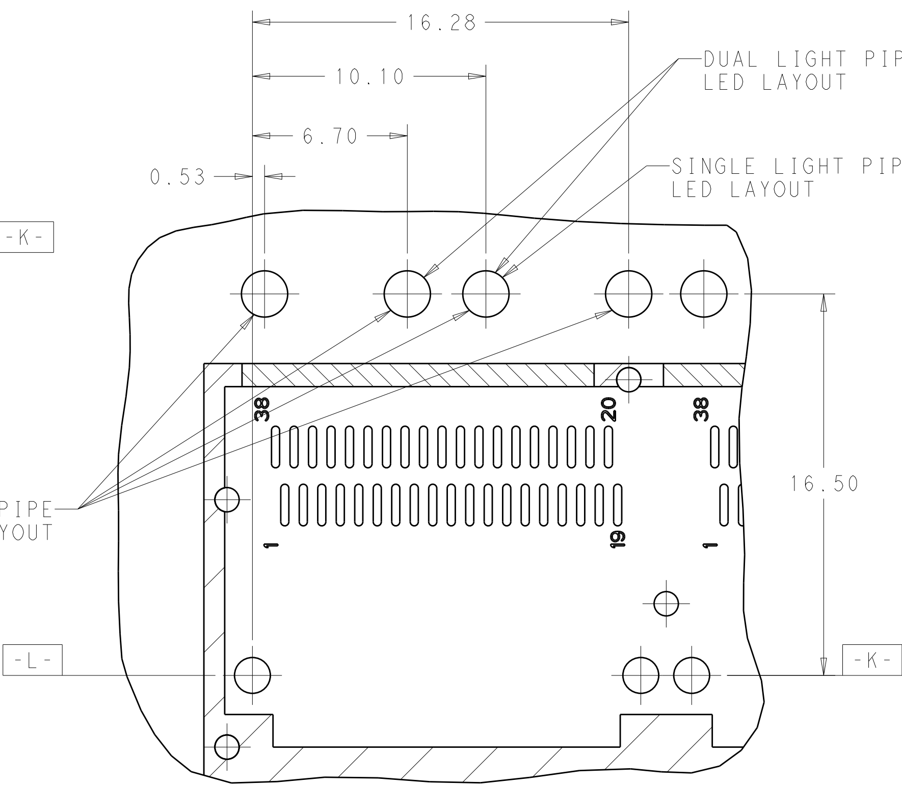
DETAIL E SCALE 6:1
