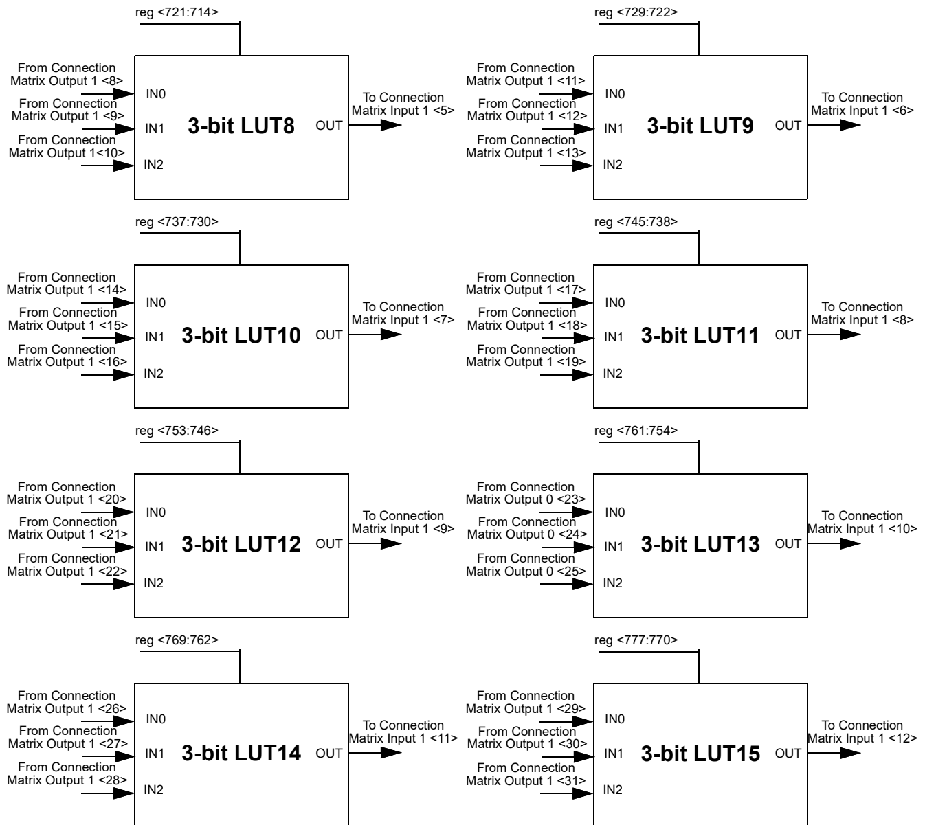
Figure 42. 3-bit LUTs
