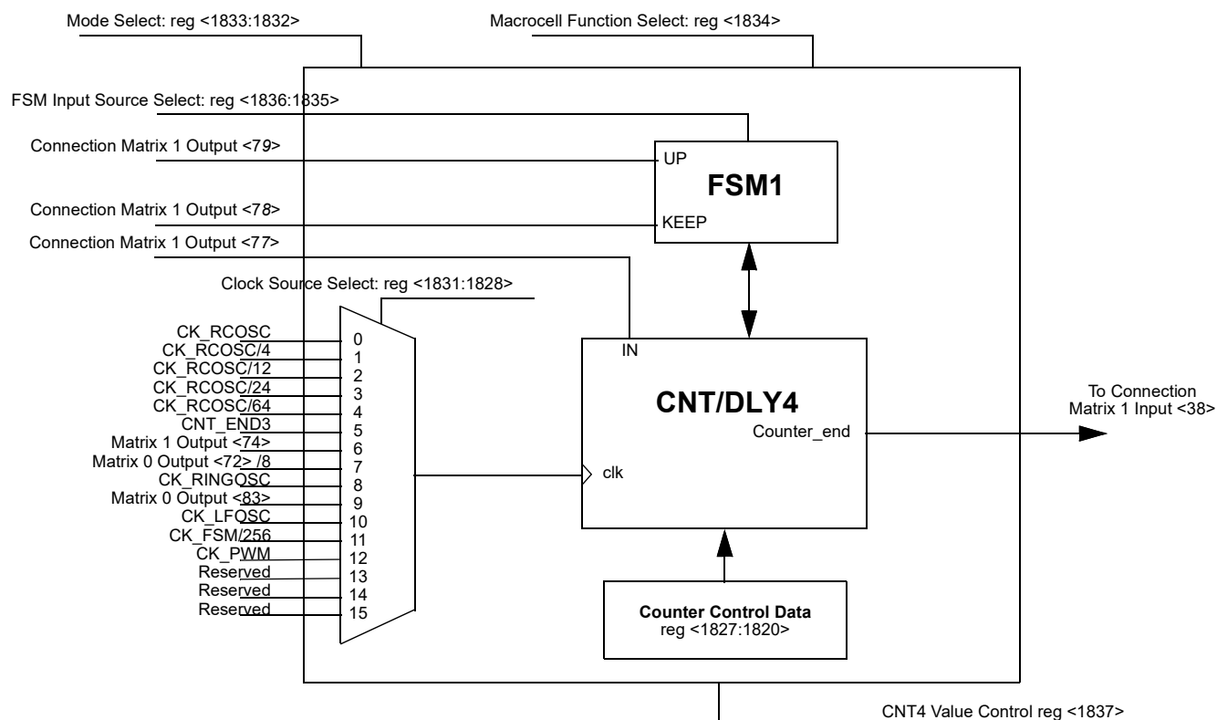
Figure 79. CNT/DLY4/FSM0
