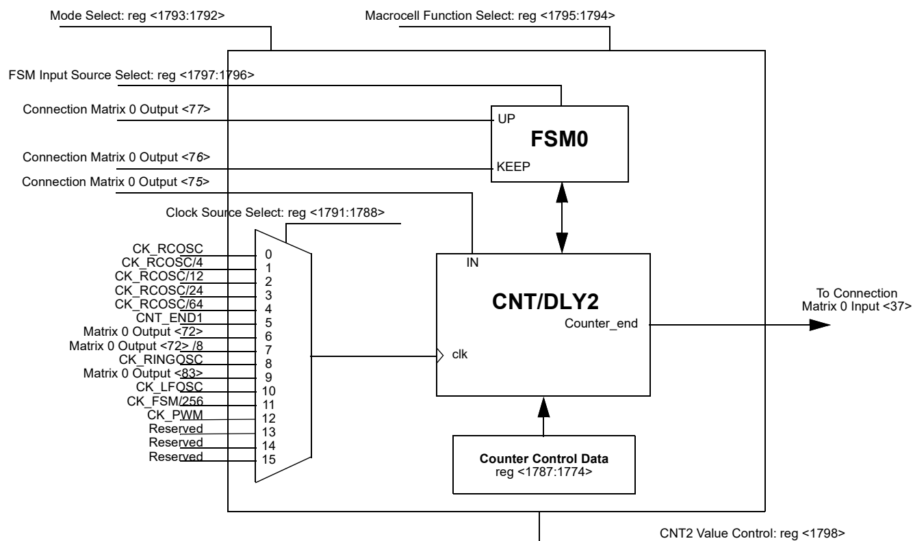
Figure 77. CNT/DLY2/FSM0
