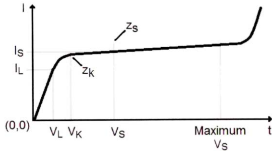
FIGURE 1 – CURRENT-REGULATOR CHARACTERISTICS
