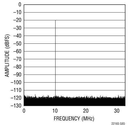
LTC2215 64k Point FFT, f_{IN} = 140.1\text{MHz} , -20dBFS, Dither "On"
