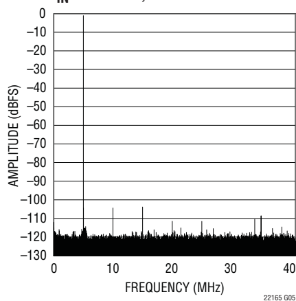
LTC2216 64k Point FFT, f_{IN} = 4.9\text{MHz} , -1dBFS
